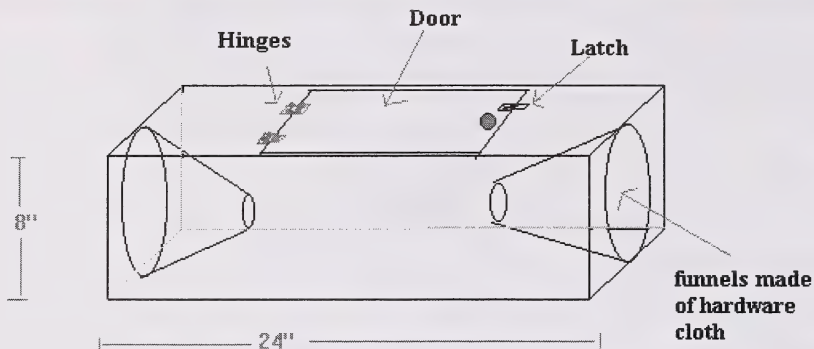
Figure 3. Funnel trap design made with quarter inch plywood.
